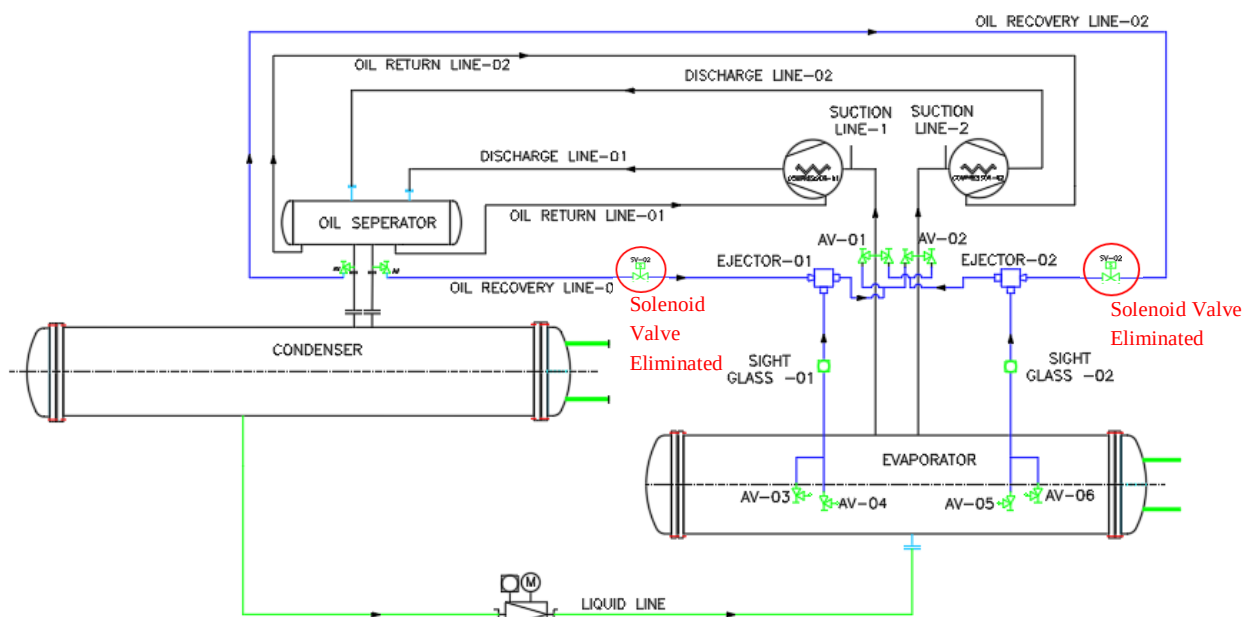
Figure 1: Improved Oil Recovery Line- Dual Compressor
