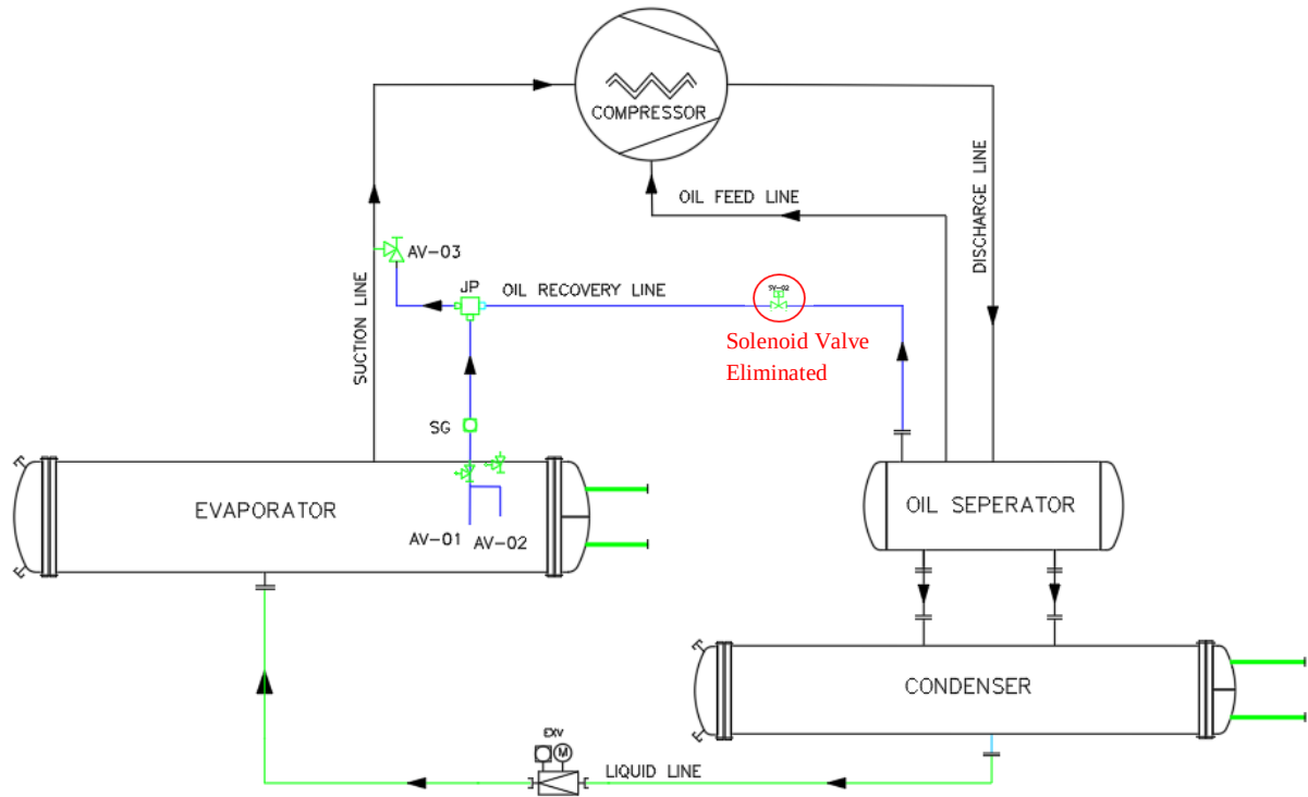
Figure 2: Improved Oil Recovery Line- Single Compressor Chiller
